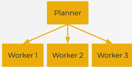
Multi-Agent
